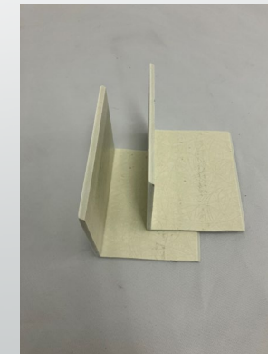
Part: FDSTAB2 3" Square connection sleeve ( For connecting pipes and elbows together use gutter glue)
